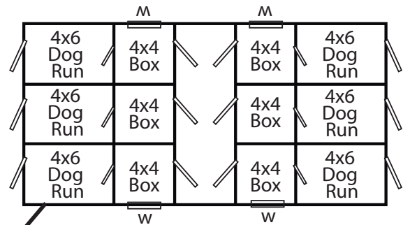
12x24 6-Run Layout
